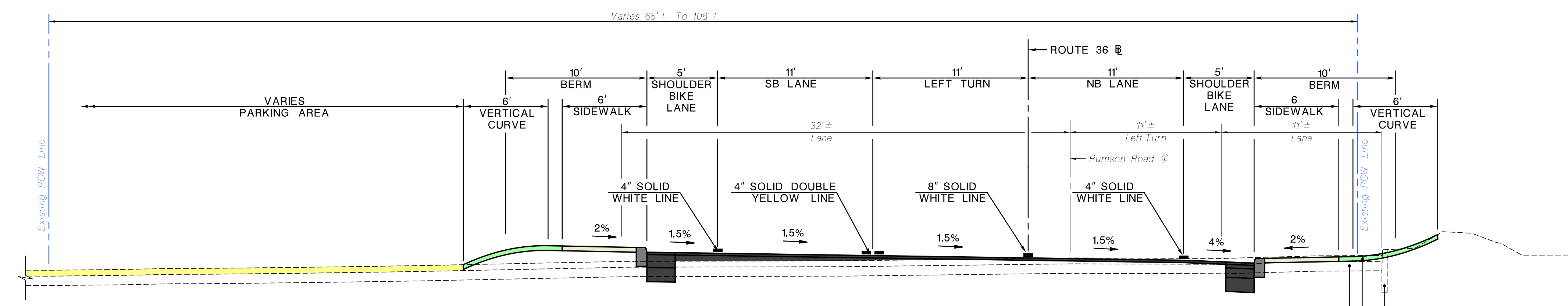
SECTION C-C ROUTE 36 NOT TO SCALE
