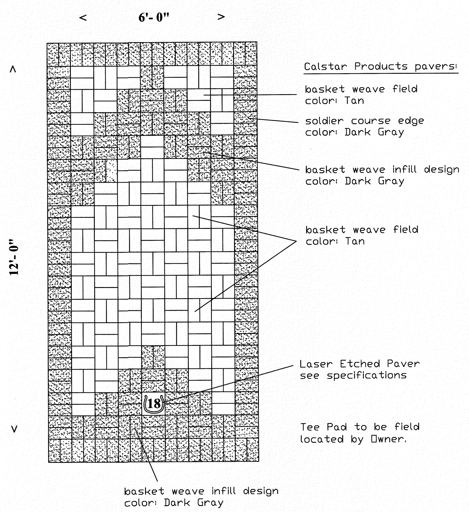
DETAIL B: Sustainable Paver Tee Pad Layout (Typical)
