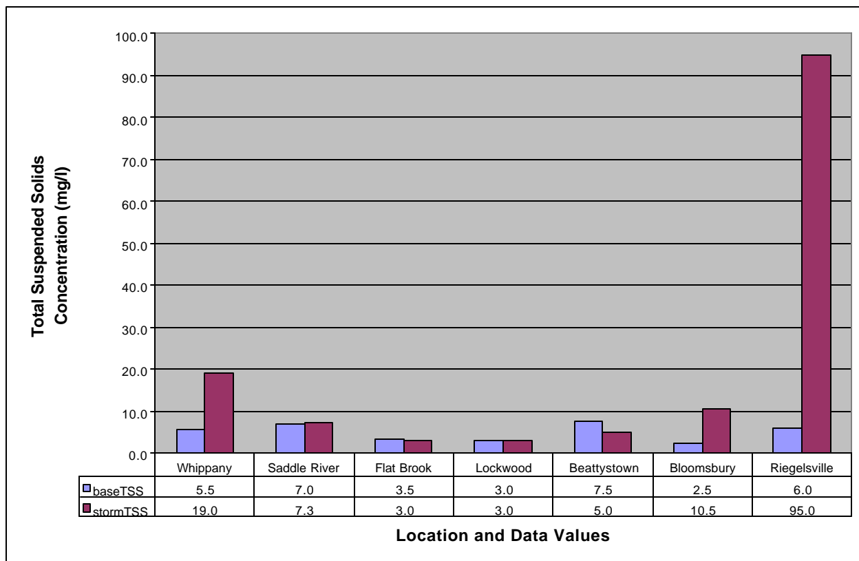
Figure 8. Total Suspended Solids Concentrations, Baseflow vs. Stormflow Conditions.
