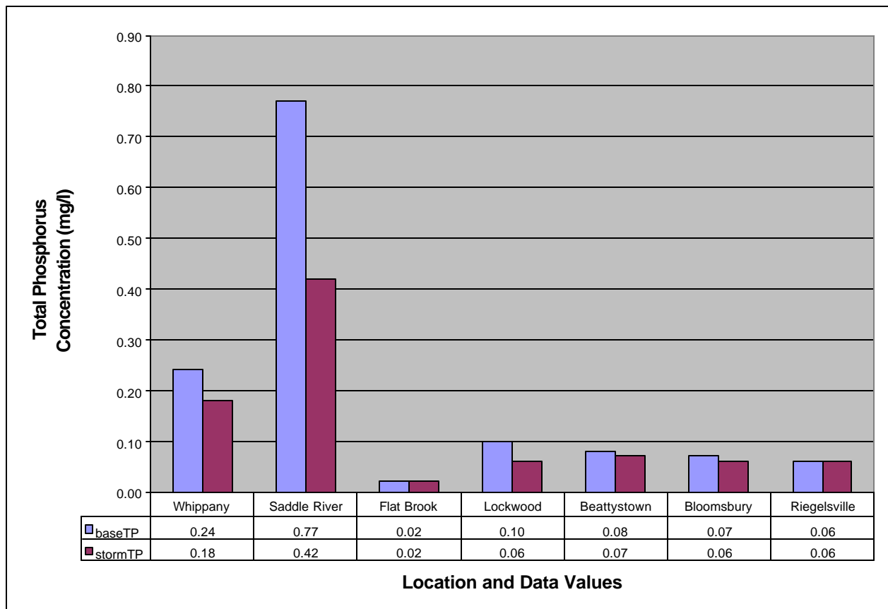
Figure 6. Total Phosphorus Concentration (mg/l), Baseflow vs. Stormflow Conditions.
