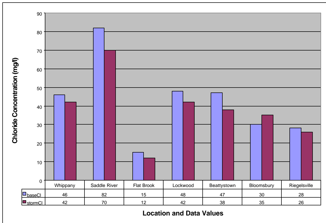
Figure 10. Chloride Concentrations, Baseflow vs. Stormflow Conditions.
