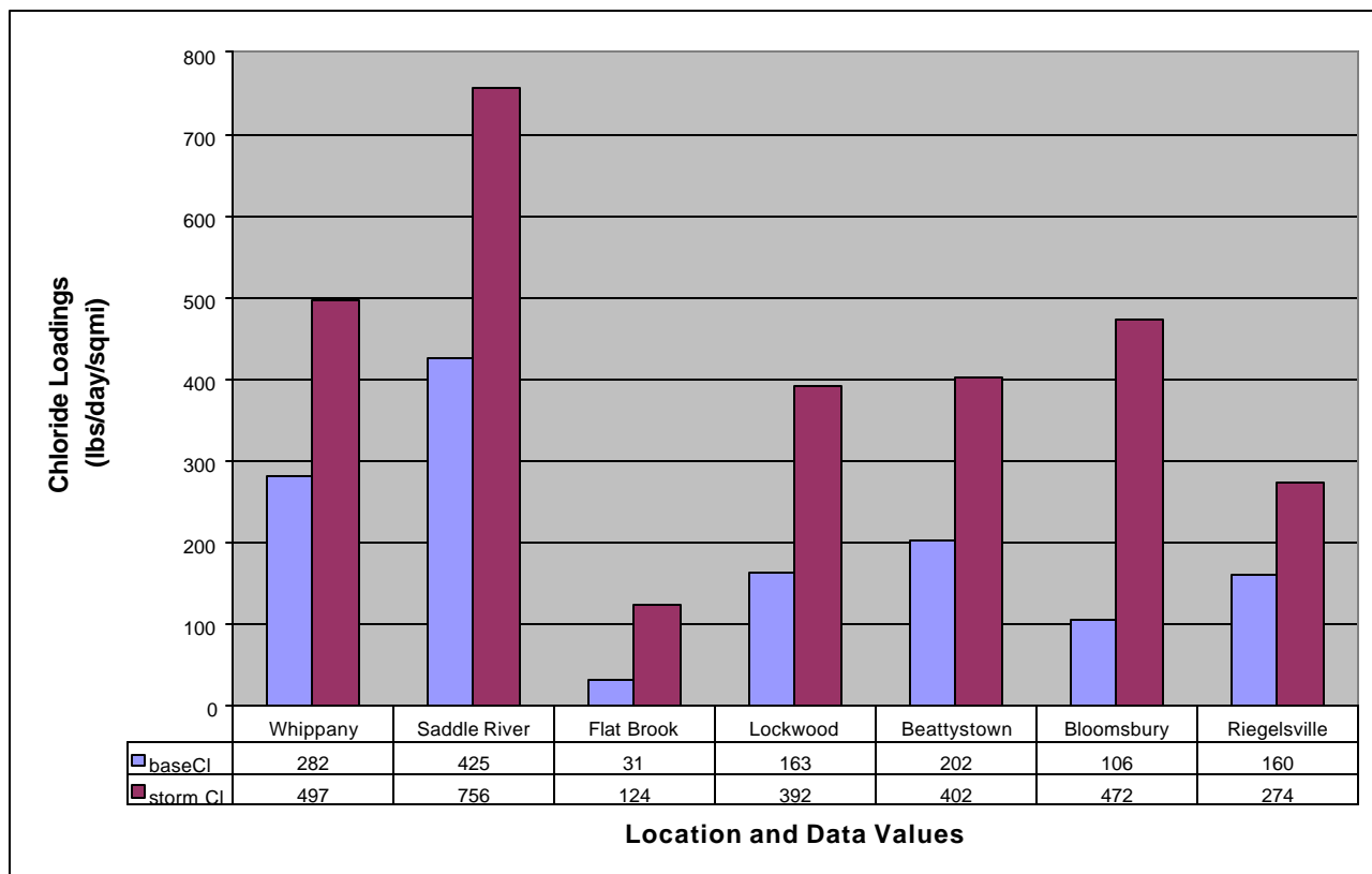
Figure 11. Chloride Loadings, Baseflow vs. Stormflow Conditions.
