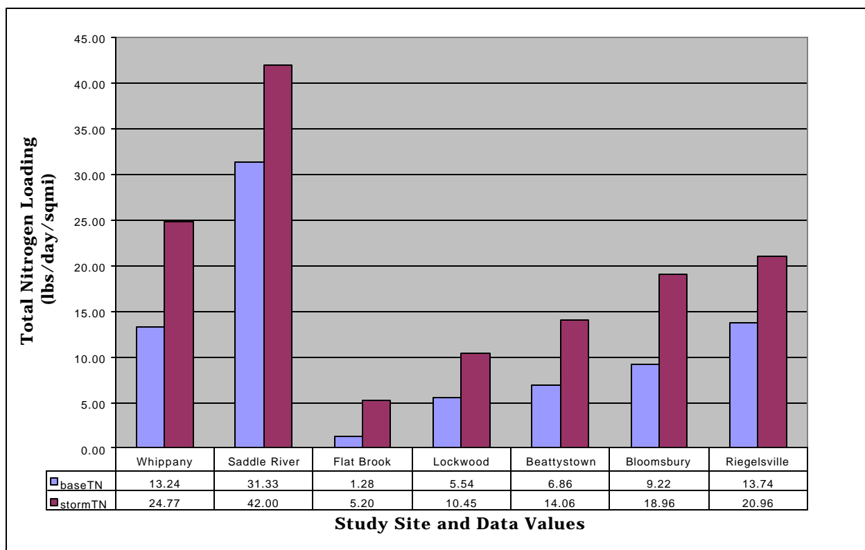
Figure 3. Total Nitrogen Loadings under Baseflow and Stormflow Conditions.
