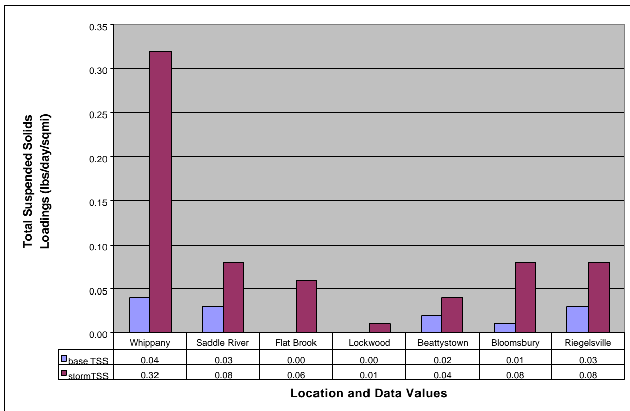
Figure 9. Total Suspended Solids Loadings, Baseflow vs. Stormflow Conditions.
