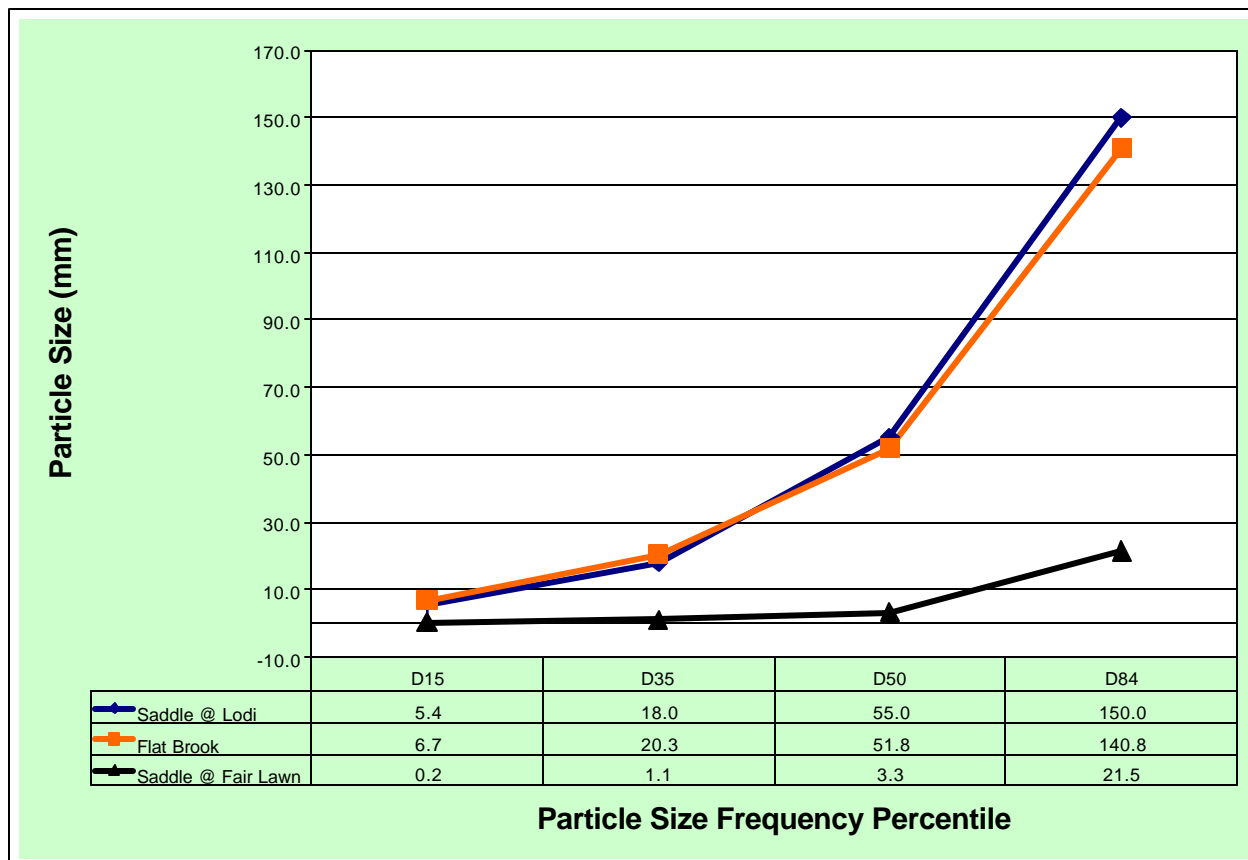
Figure 12. Comparison of particle size distributions sampled from the Saddle River at Lodi, NJ; Saddle River at Fair Lawn, NJ; and the Flat Brook reference reach.
