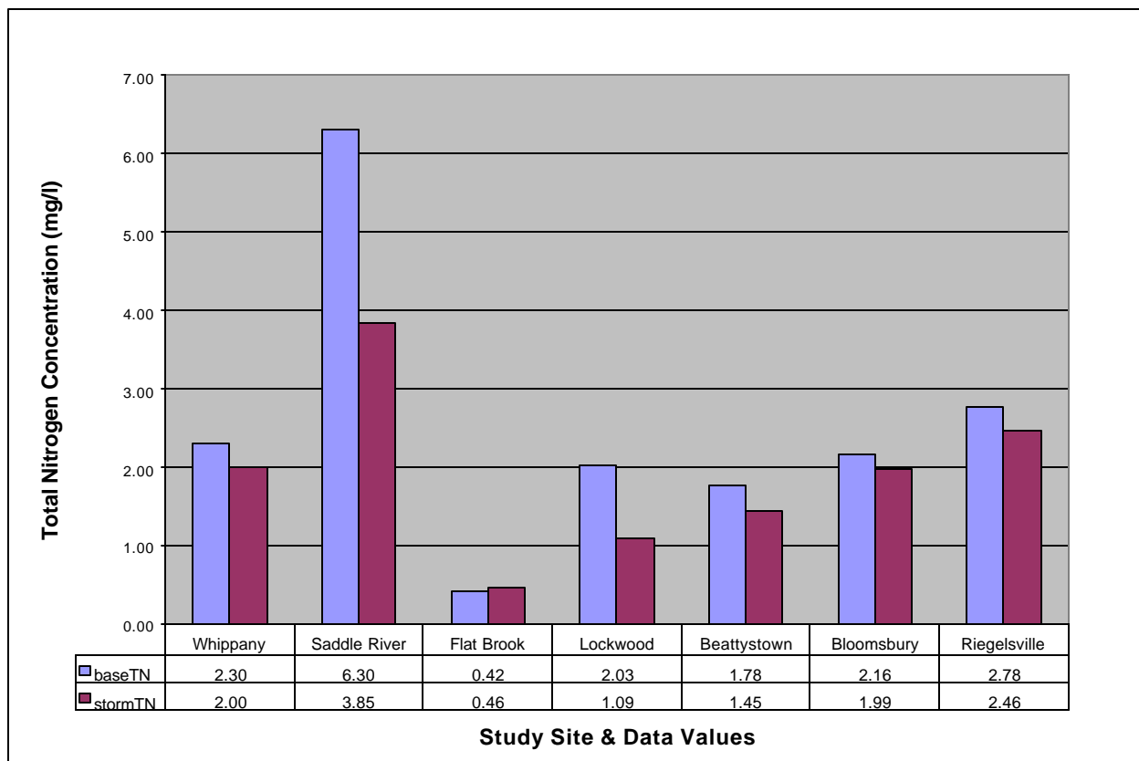
Figure 2. Total Nitrogen Concentrations under Baseflow and Stormflow Conditions.
