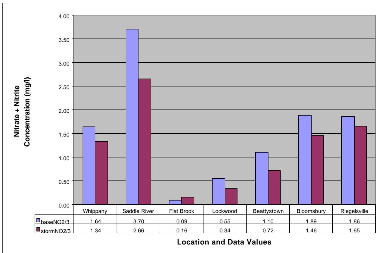
Figure 4. Nitrate plus Nitrite Concentrations under Baseflow vs. Stormflow Conditions.
